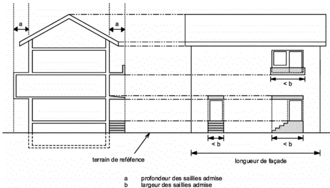
Figure 2.3.b Saillies (façade)
