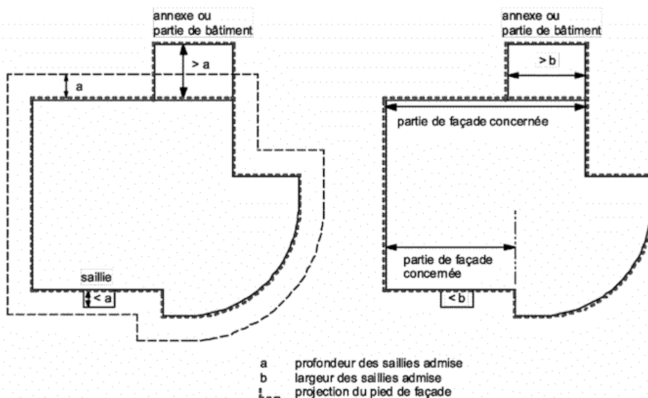
Figure 2.3.a Saillies (coupe)
