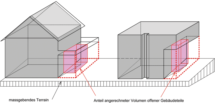
Figur 8.3 Baumassenziffer
