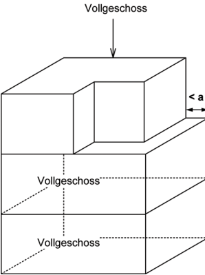
Figur 6.4 Attikageschosse
